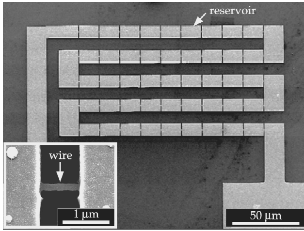
FIG. 2. 50 wires with a length of 840 nm and a width of 140 nm each with large, thick thermal reservoirs in between, were fabricated using the technique illustrated in Fig. 1. The inset shows one single wire.
