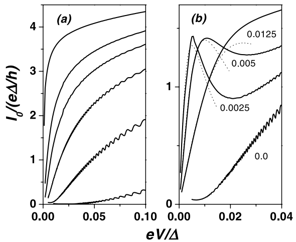
Fig. 5. Low bias current–voltage characteristic for the symmetric case. Panel (a) corresponds to the fully phase-coherent case ( \eta = 0 ) and different values of \Gamma^*/\Delta = 10, 5, 4, 3, 2, 1 from top to bottom. Panel (b) corresponds to \Gamma^*/\Delta = 2 and different values of \eta/\Delta as indicated. The dotted lines show the analytic description of the eV < \eta regime given by Eq. (11).
