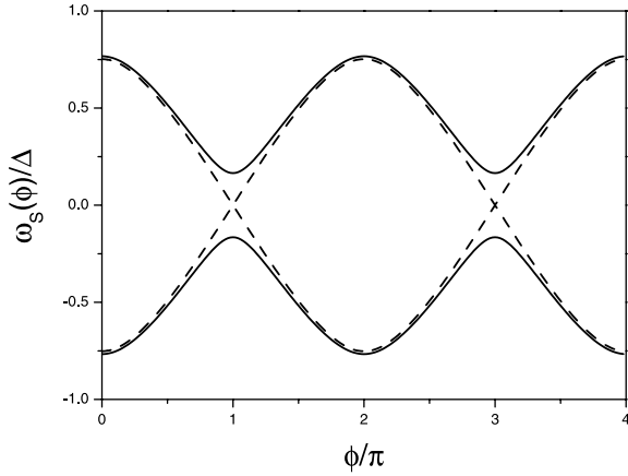
Fig. 4. Andreev states for a S-QD-S in the Kondo regime. Dashed and full lines correspond to a symmetric and non-symmetric situation, respectively.
