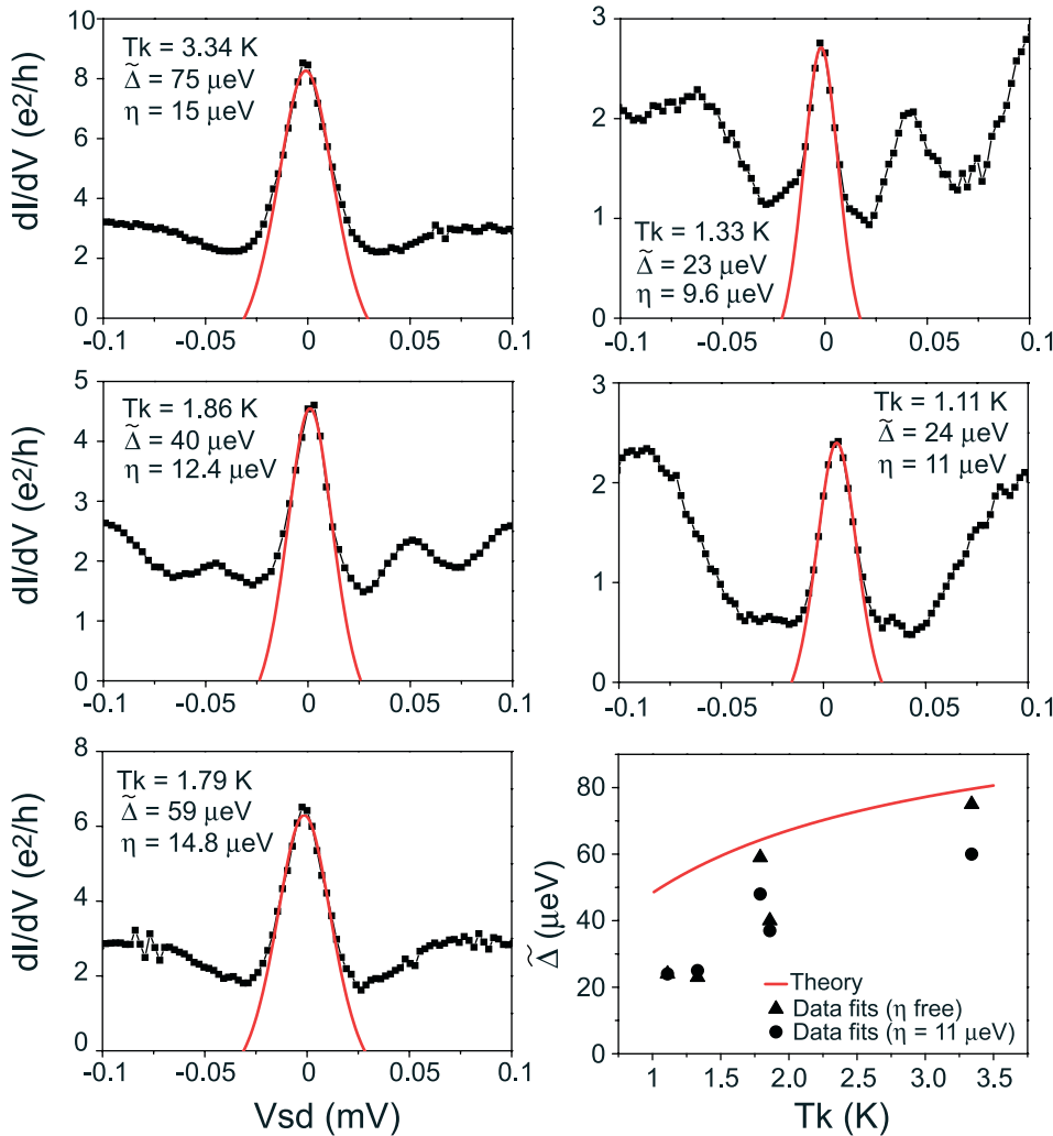
Fig. 6. Differential conductance in the middle of five different Kondo ridges with decreasing T_K . The red lines are fits to the data using Eq. (11). The lower right panel shows the fitted values of \tilde{\Delta} vs T_K compared to the theoretical prediction \tilde{\Delta}/\Delta \approx 1/(1 + \Delta/T_K) .
